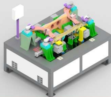
MULTILINK SUBFRAME PIERCING MACHINE
