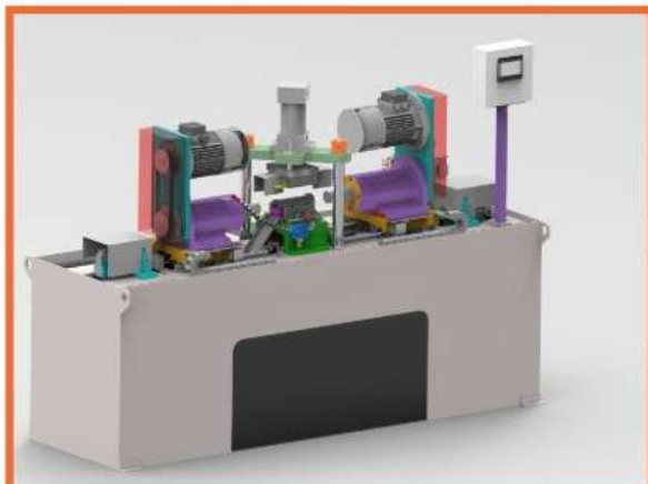
HEADER TUBE BORING MACHINE
